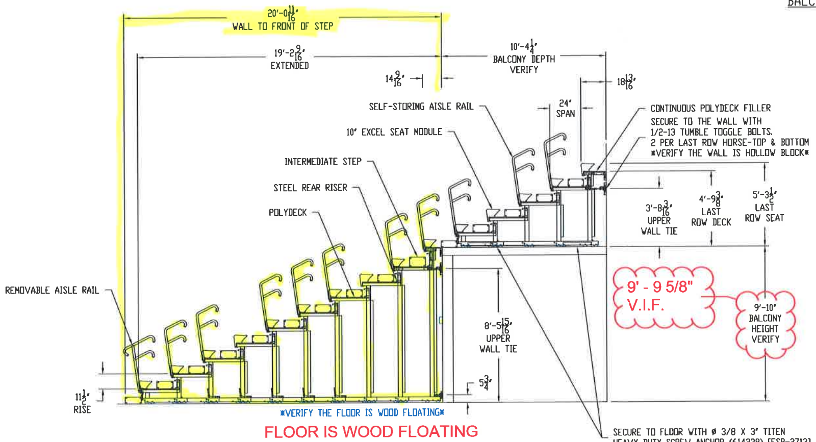
15 ROW SIDE ELEVATION BANK #1 - 10 ROW TELESCOPIC BANK #2 - 5 ROW FIXED OPEN
