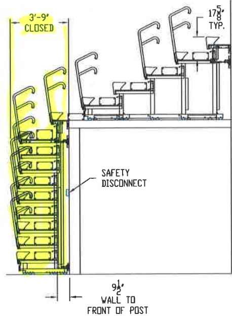
CLOSED VIEW
