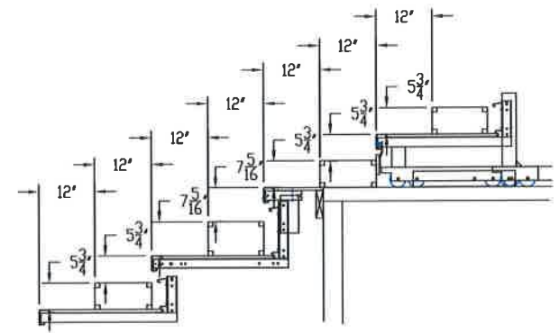
BALCONY ACCESS DETAIL
